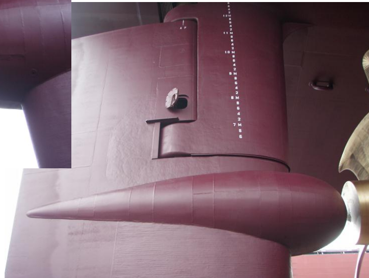
Rudder bulb on Danaos 8500 teu vessels built in Jiangnan shipyard
